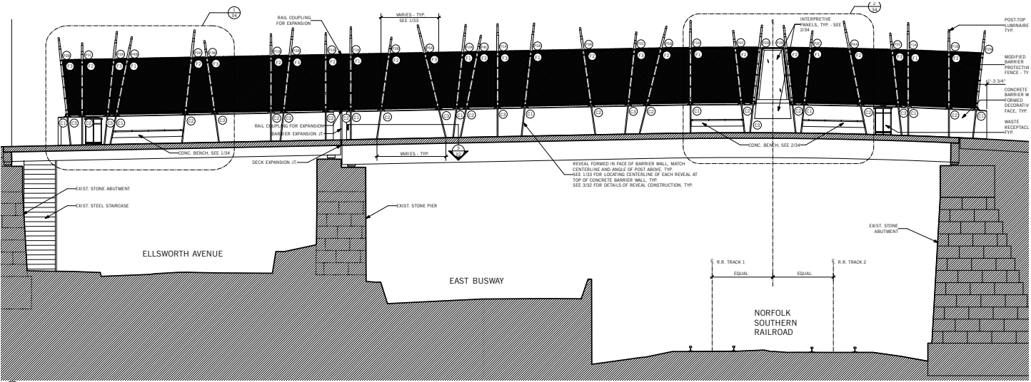
17 ELEVATION OF BARRIER AND PROTECTIVE FENCE (OPP. SIDE SIGN) Scale: 1/4" = 1'-0"
